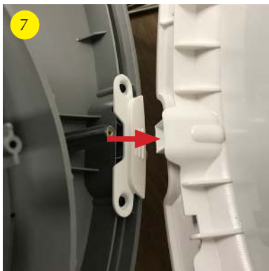
7 To re-install front cover, position bottom pin over slot. Let magnet re-engage.
